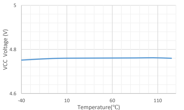
Figure 13. VCC Voltage vs Temperature
