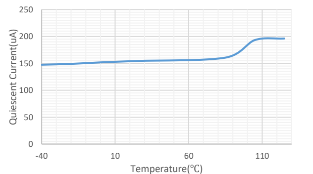
Figure 11. Quiescent Current vs Temperature
