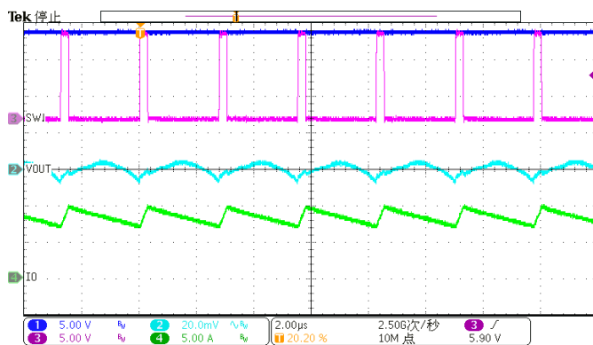
Figure 27. Output Ripple (Iload=8A) 400kHz
