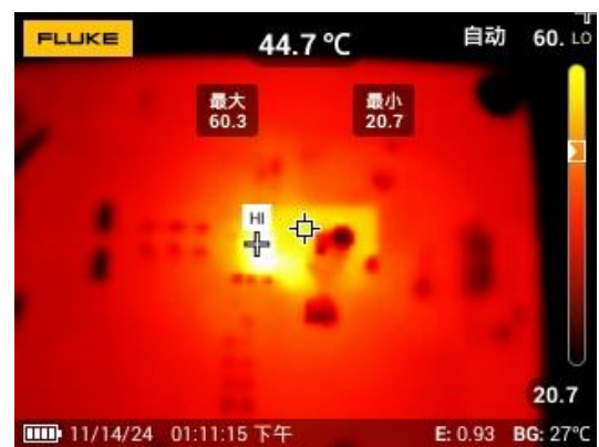
Figure 32. Thermal, Fsw=400kHz, Iload=8A
